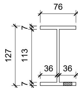
SCALE 1:5
