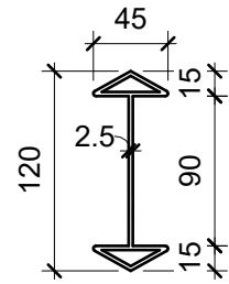
SCALE 1:5
