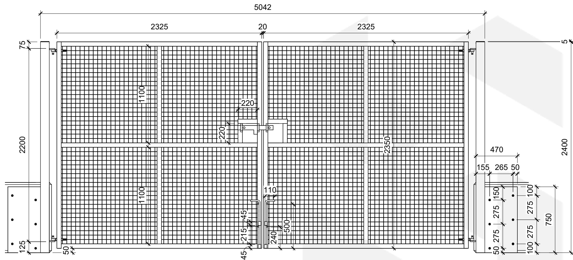
SCALE 1:25
